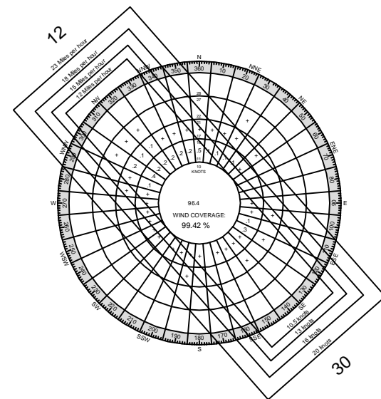
ALL WEATHER WIND ROSE
