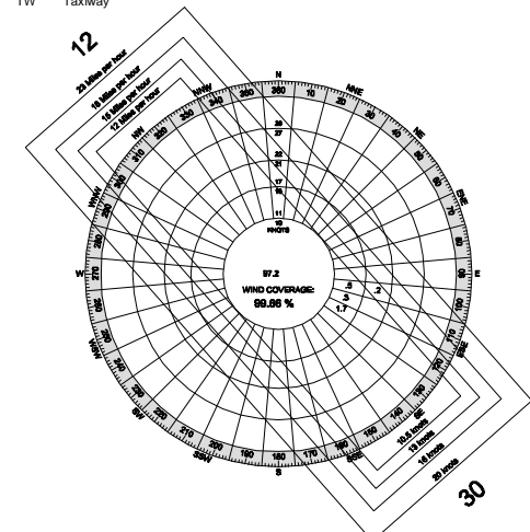
IFR WIND ROSE
