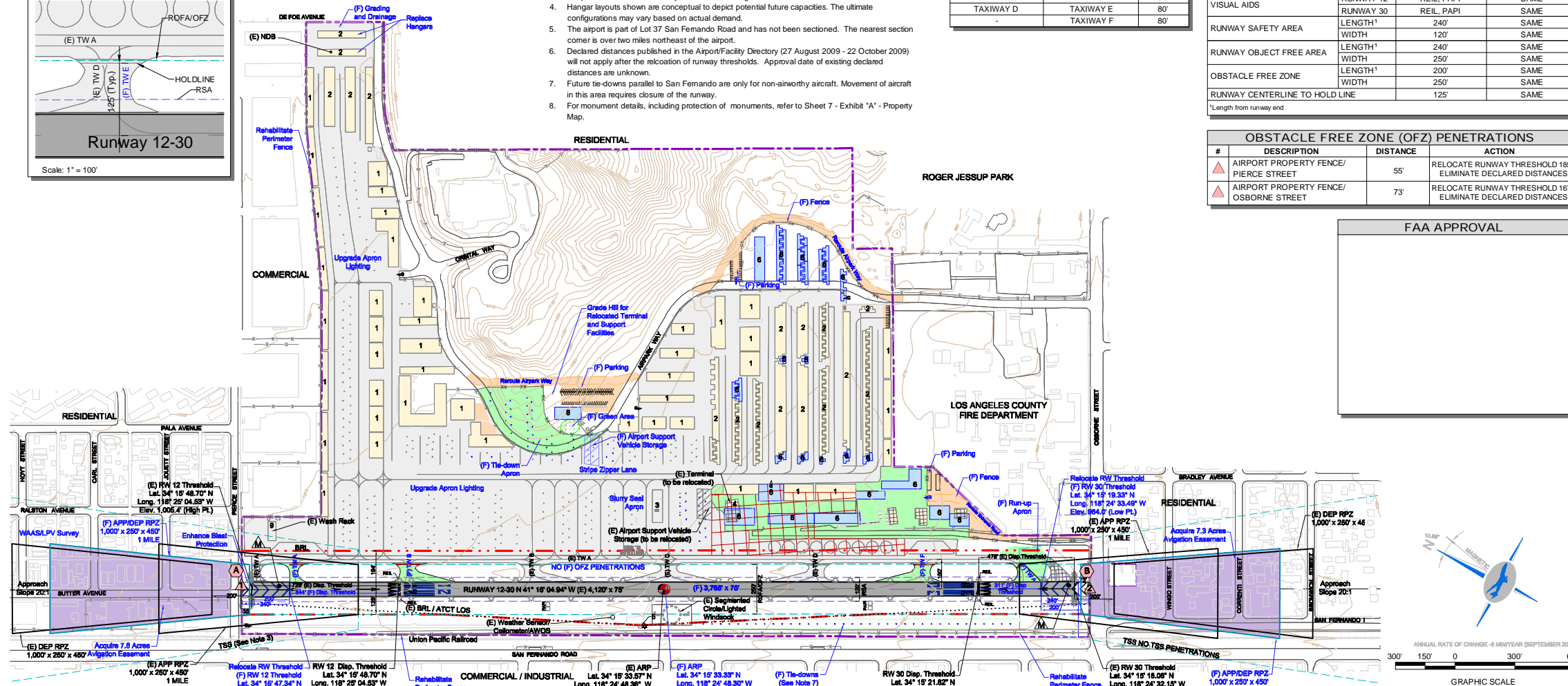
Figure 7-1 Airport Layout Plan
