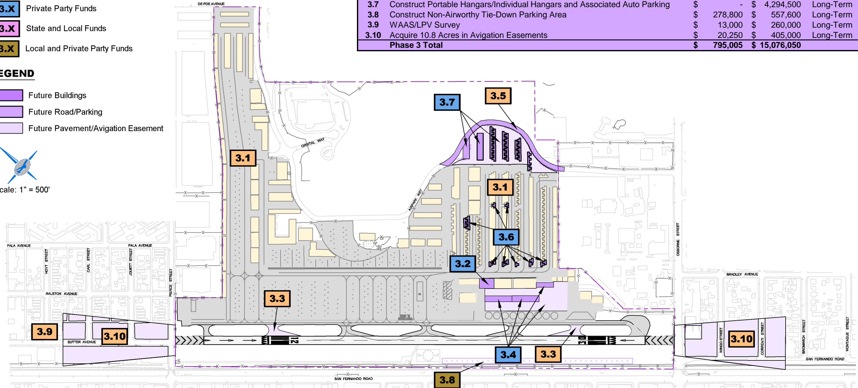
Figure 8-3 Phase 3 Improvements
