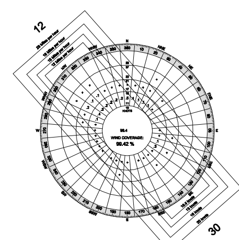
ALL WEATHER WIND ROSE
