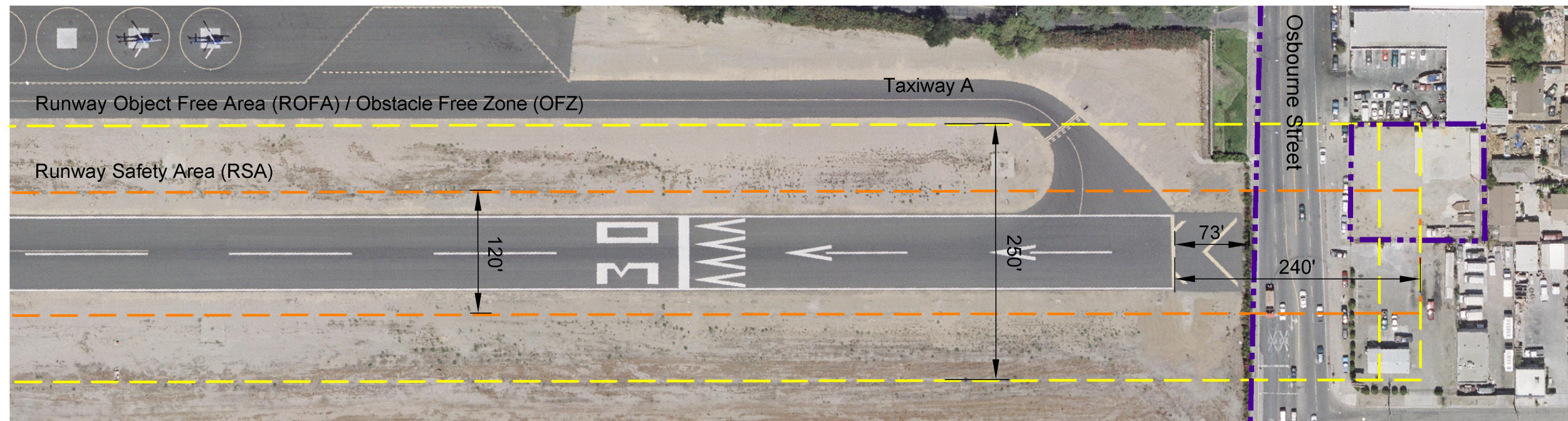
Runway 30
