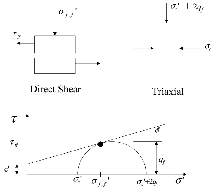
Figure 7.1. Stress States at Failure in Direct Shear and Triaxial CD Tests
