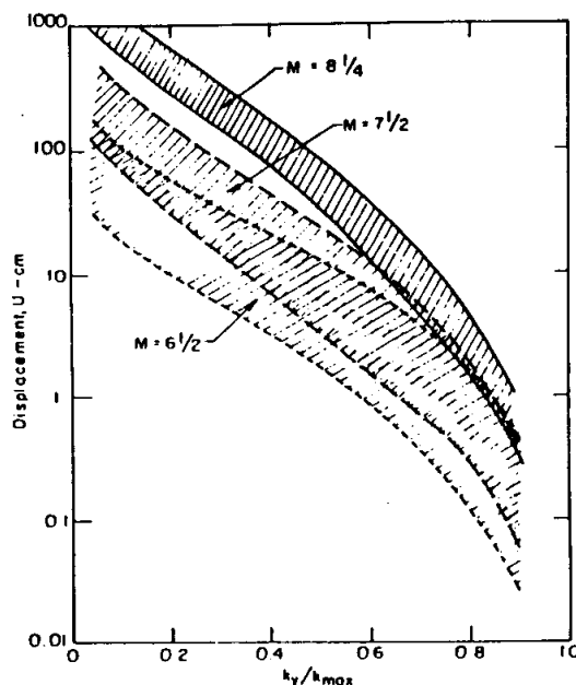
Fig. 11.6. Variation of Slope Displacement with Magnitude and k_y/k_{max} (Makdisi and Seed, 1978).
