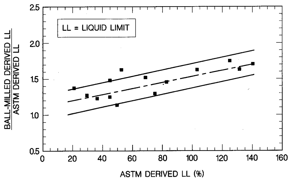
Figure 7.5e. Ratio for Ball-Milled and ASTM Values of Liquid Limit (Stark and McCone, 2001)
