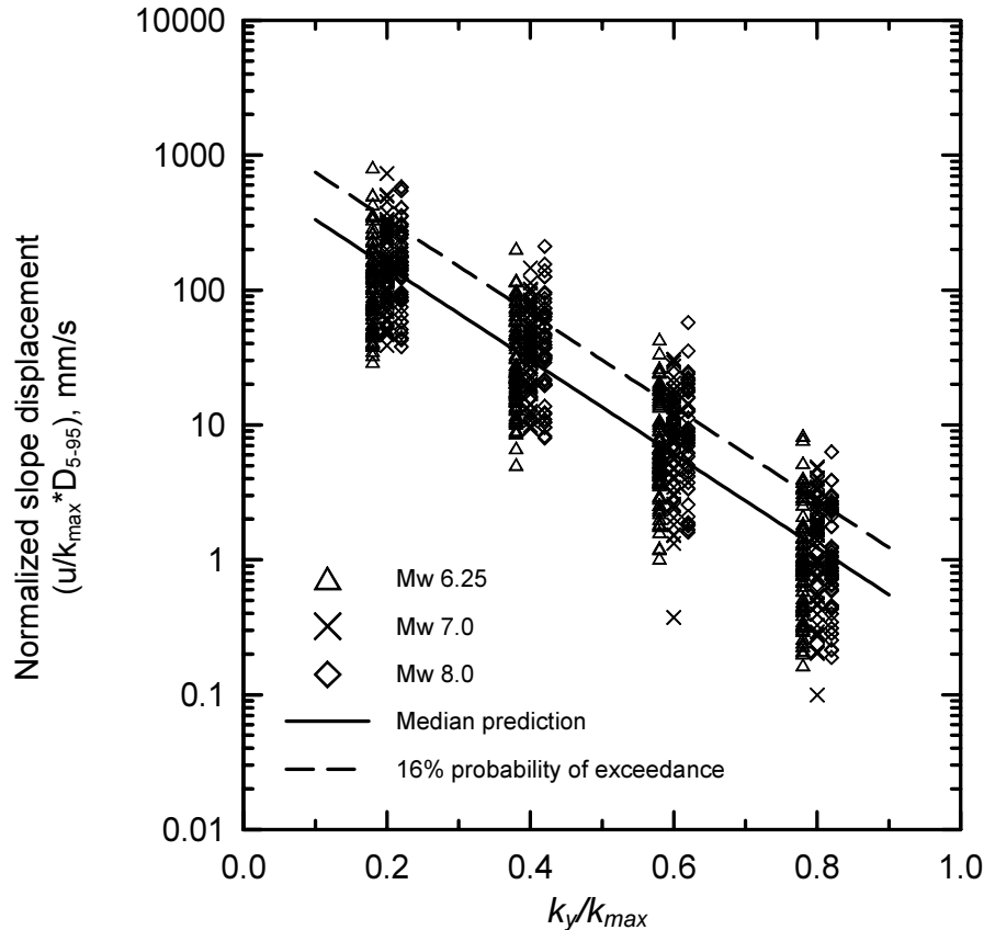
Fig. 2. Normalized Sliding Displacement (modified from Bray and Rathje, 1998).
