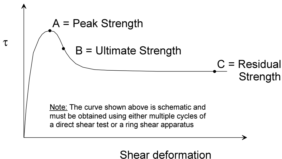
Figure 7.4. Diagrammatic Stress-Displacement Curve
