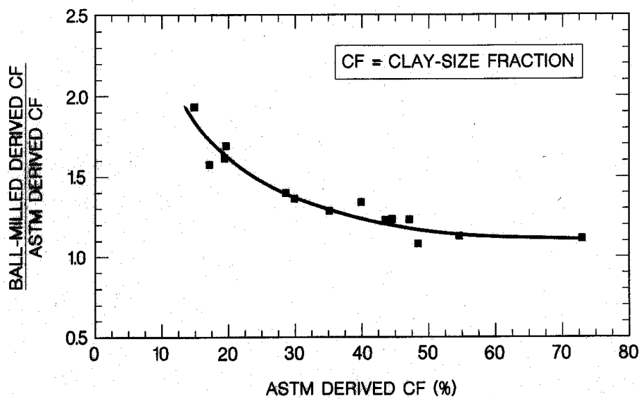
Figure 7.5f. Ratio of Ball-Milled and ASTM Values of Clay-Size Fraction (Stark and McCone, 2001)
