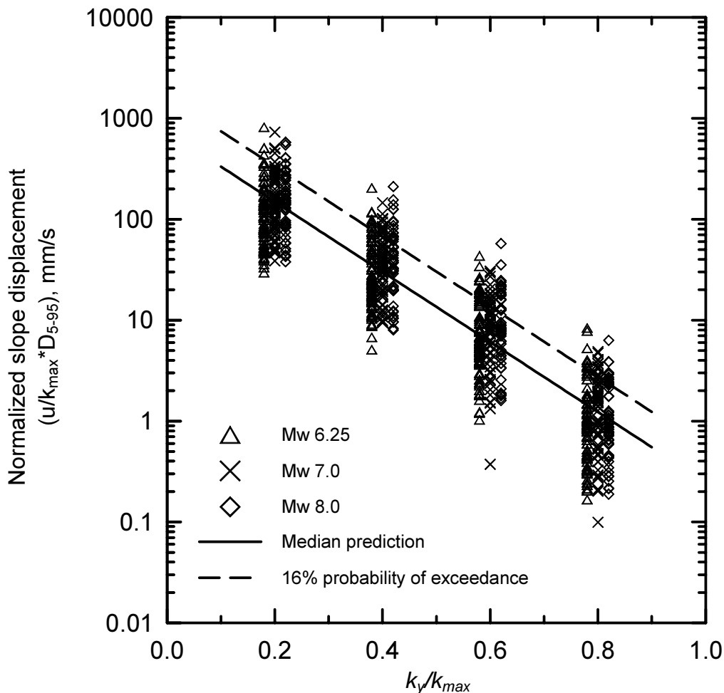
Figure 11.4. Normalized Sliding Displacement (modified from Bray et al., 1998).
