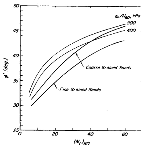
Figure 7.5a. Empirical Correlation Between Friction Angle of Sand and Normalized Standard Penetration Blow Count (Terzaghi et al., 1996)
