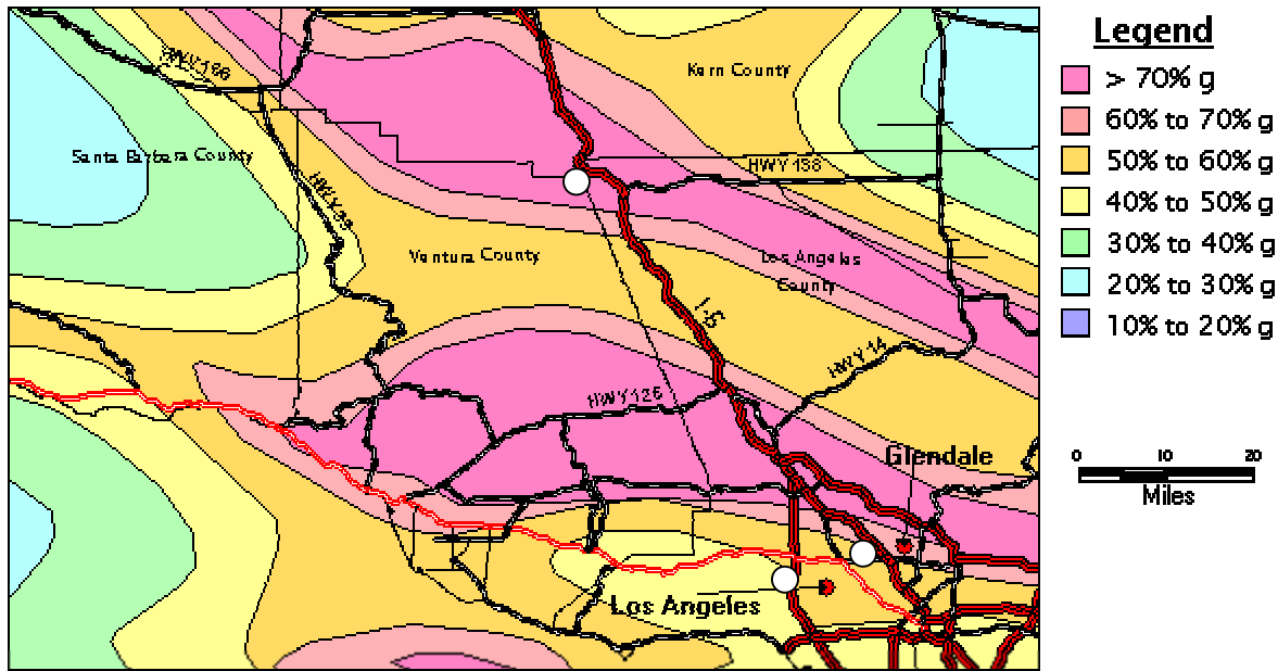
Fig. 5. Probabilistic Seismic Hazard Map by Petersen et al. (1996) for MHA on Soft Rock Site Condition at the 475-Year Hazard Level.
