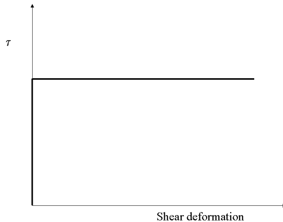
Figure 7.3. Depiction of Rigid Perfectly Plastic Soil Stress-Deformation Response
