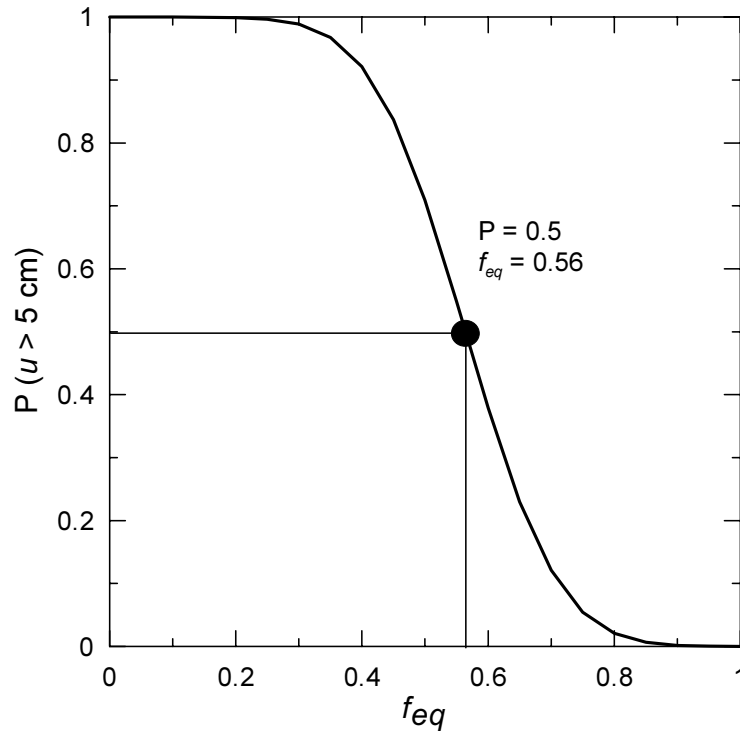
Fig. 3. Variation of Exceedance Probability for 5 cm Slope Displacement with f_{eq} for M = 7 , r = 20 km, and MHA_r = 0.4g
