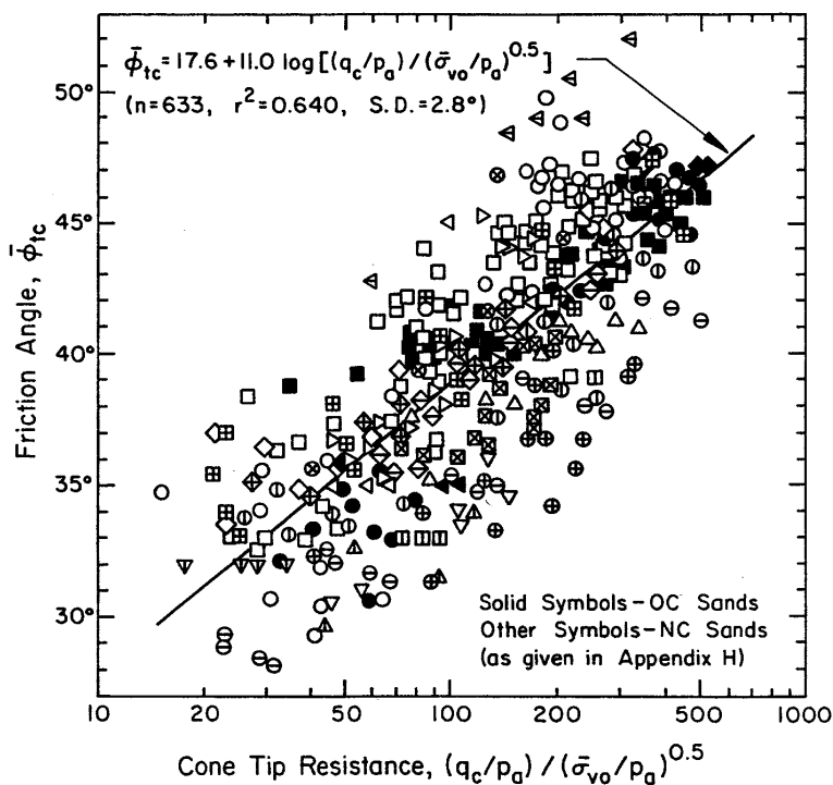
Figure 7.5b. Empirical Correlation Between Friction Angle of Sand and Normalized CPT Tip Resistance (Kulhawy and Mayne, 1990)
