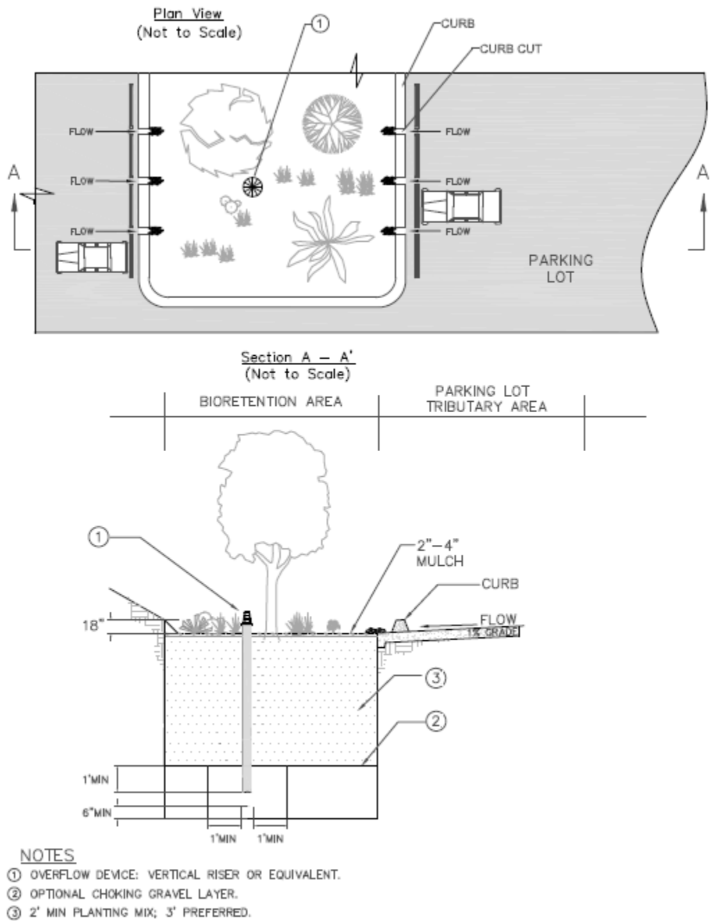
Figure E-1. Bioretention Area Schematic
