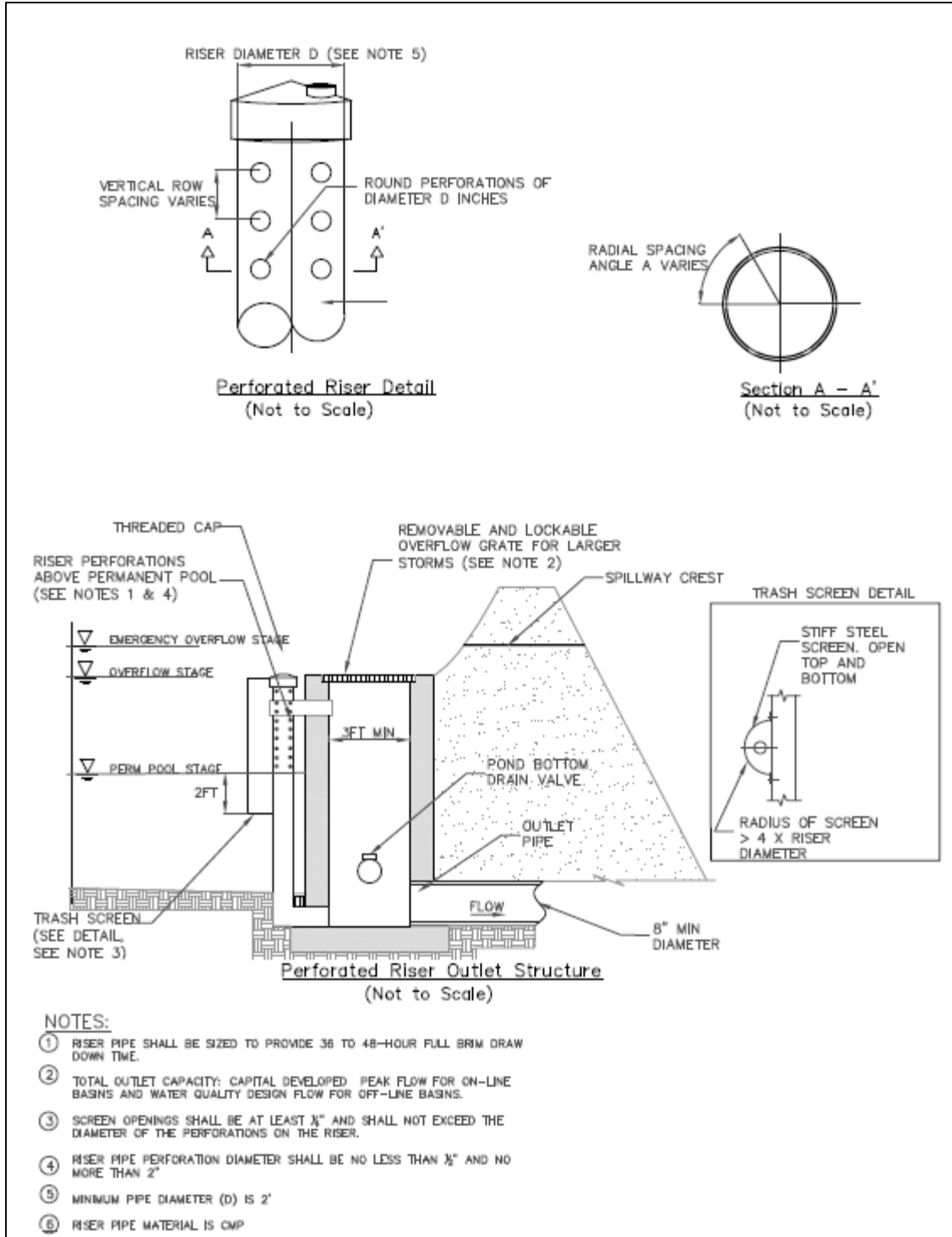
Figure E-19. Perforated Riser Structure
